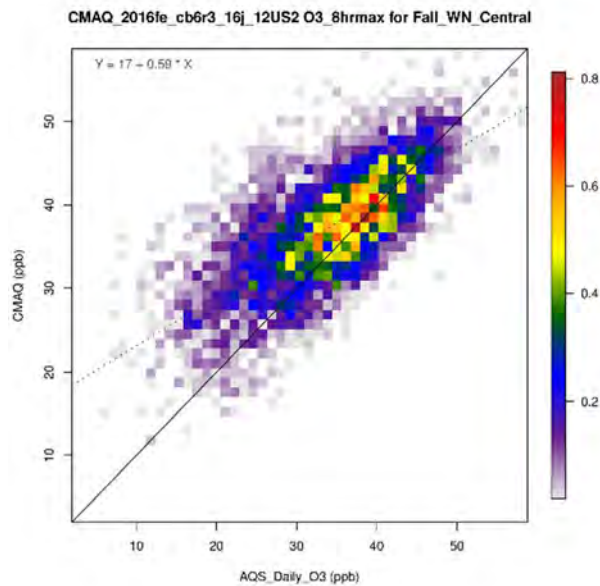
5 Figure 2B-10. Density scatter plots of observed versus predicted MDA8 O 3 from the 12km 6 resolution CONUS simulation for the WestNorthCentral region by season. 7 Each plot has a separate scale that is shared for the x and y axes. The dashed line 8 represents the best fit linear regression line.
