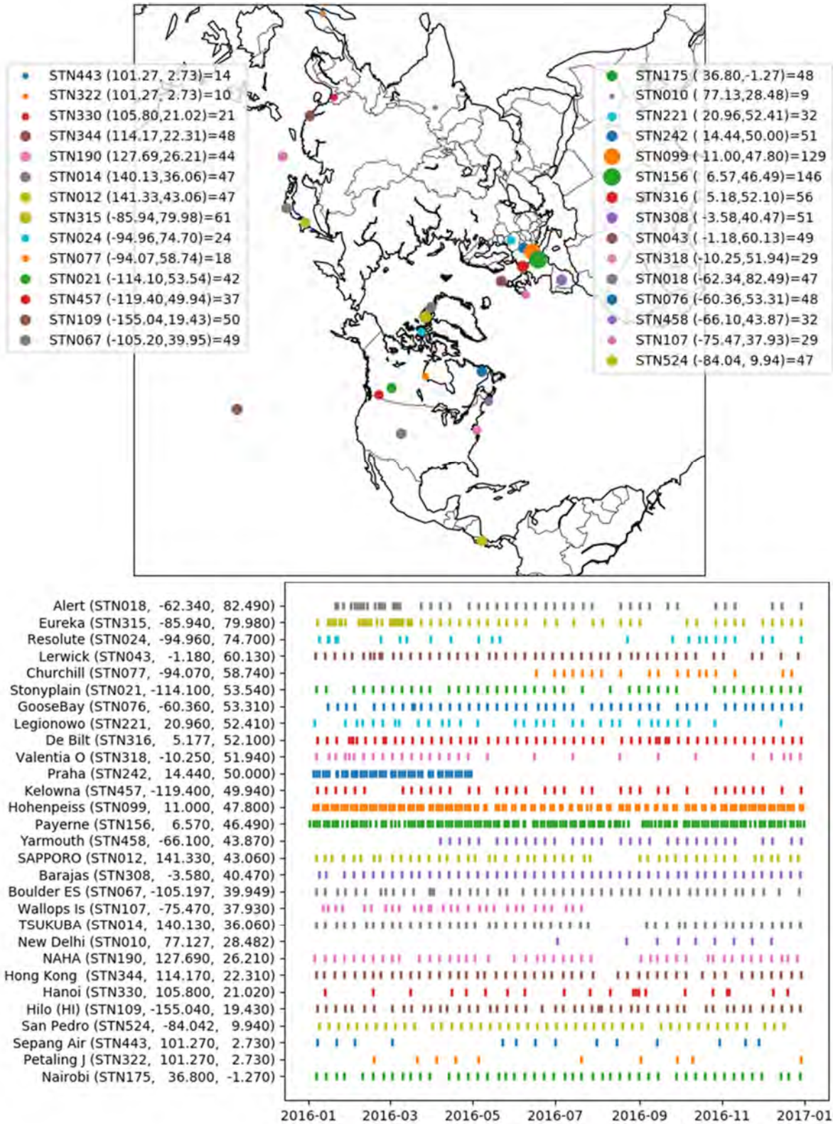
1 Figure 2B-17. WUDEC sonde locations and sampling frequency used in evaluation of 2 hemispheric model simulation.
