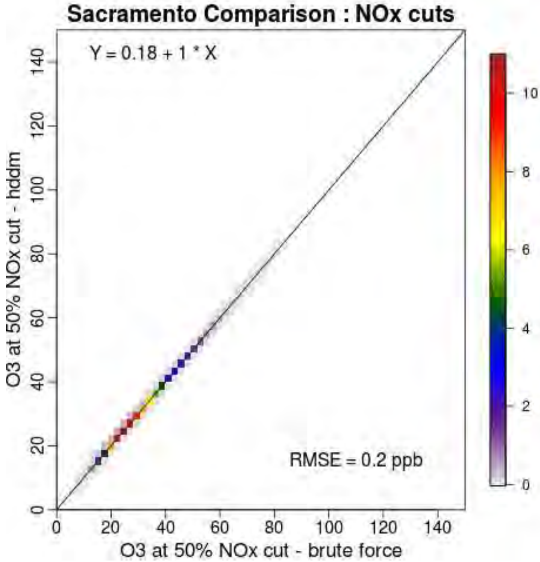
2 Figure 3C-56. Comparison of brute force and 3-step HDDM O 3 estimates for 50% NO x 3 cut conditions in Sacramento.
