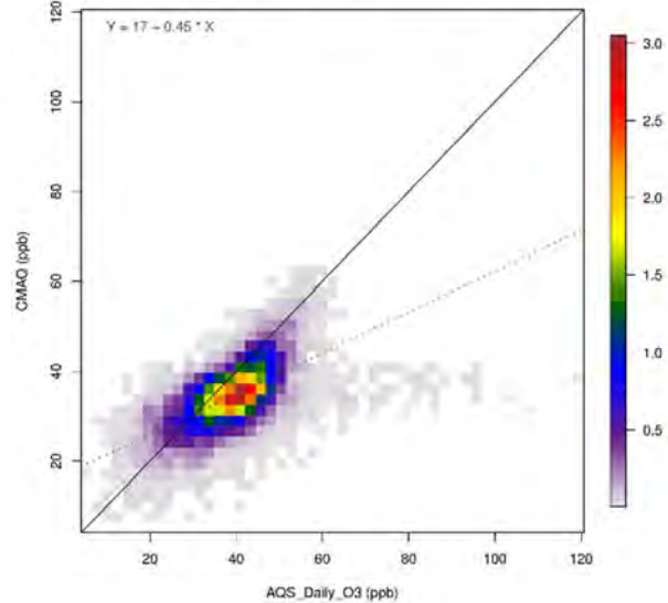
CMAQ_2016fe_cb6r3_16j_12US2 O3_8hrmax for Winter_Southwest
