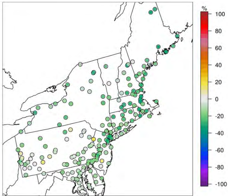
1 2 Figure 3C-13. Normalized mean bias for MDA8 O 3 in the Northeastern U.S., spring 2016.
