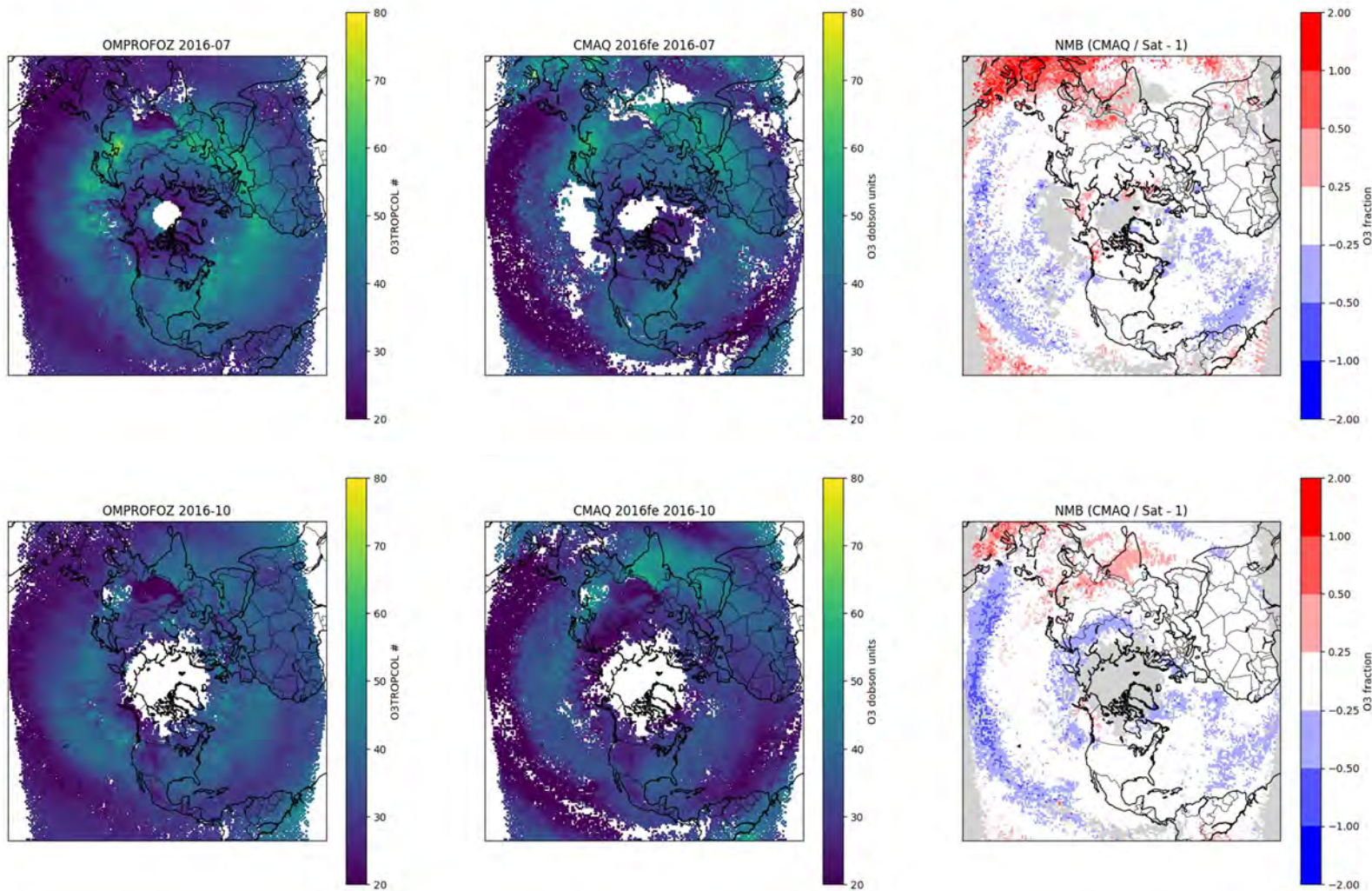
3 Figure 2B-23. OMI O 3 (OMPROFOZ v003, left) compared to simulated (hemispheric CMAQ simulation, center), and ratios 4 (right) of vertical column densities for July (top), and October (bottom).
