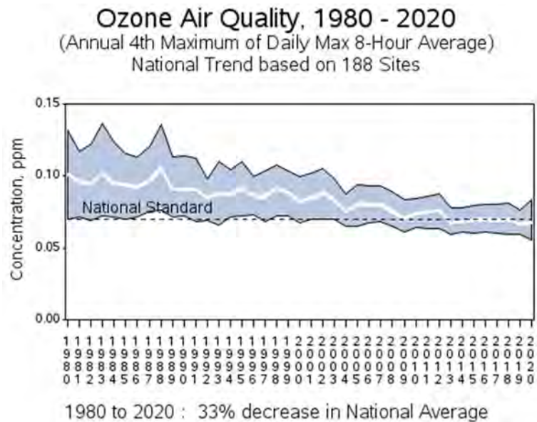
Figure 2-10. National trend in annual 4 th highest MDA8 values, 1980 to 2020. The white center line is the average while the filled area represents the range between the 10 th and 90 th percentiles. The dotted line is the level of the standard.
