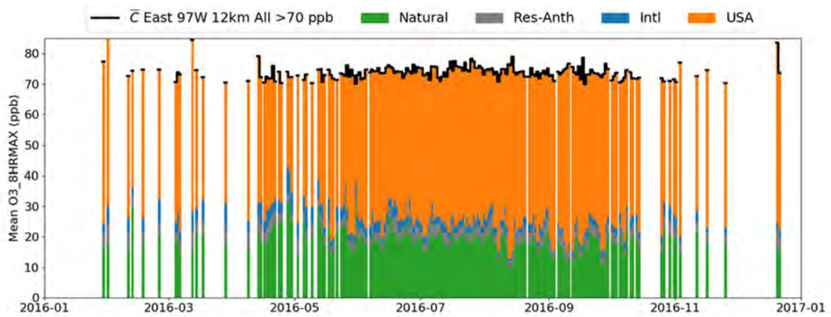
Figure 2-28. Annual time series of regional average predicted MDA8 O 3 and contributions of each source to predicted MDA8 total O 3 (see legend) in the West (top) and East (bottom) including only those grid-cell days with MDA8 greater than 70 ppb. Natural is global natural sources, Intl is international anthropogenic sources, USA is U.S. anthropogenic sources, and Res-Anth is the residual anthropogenic (see Table 2-2 for further descriptions).
