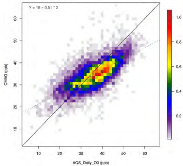
CMAQ_2016fe_cb6r3_16j_12US2 O3_8hrmax for Winter_Southeast
