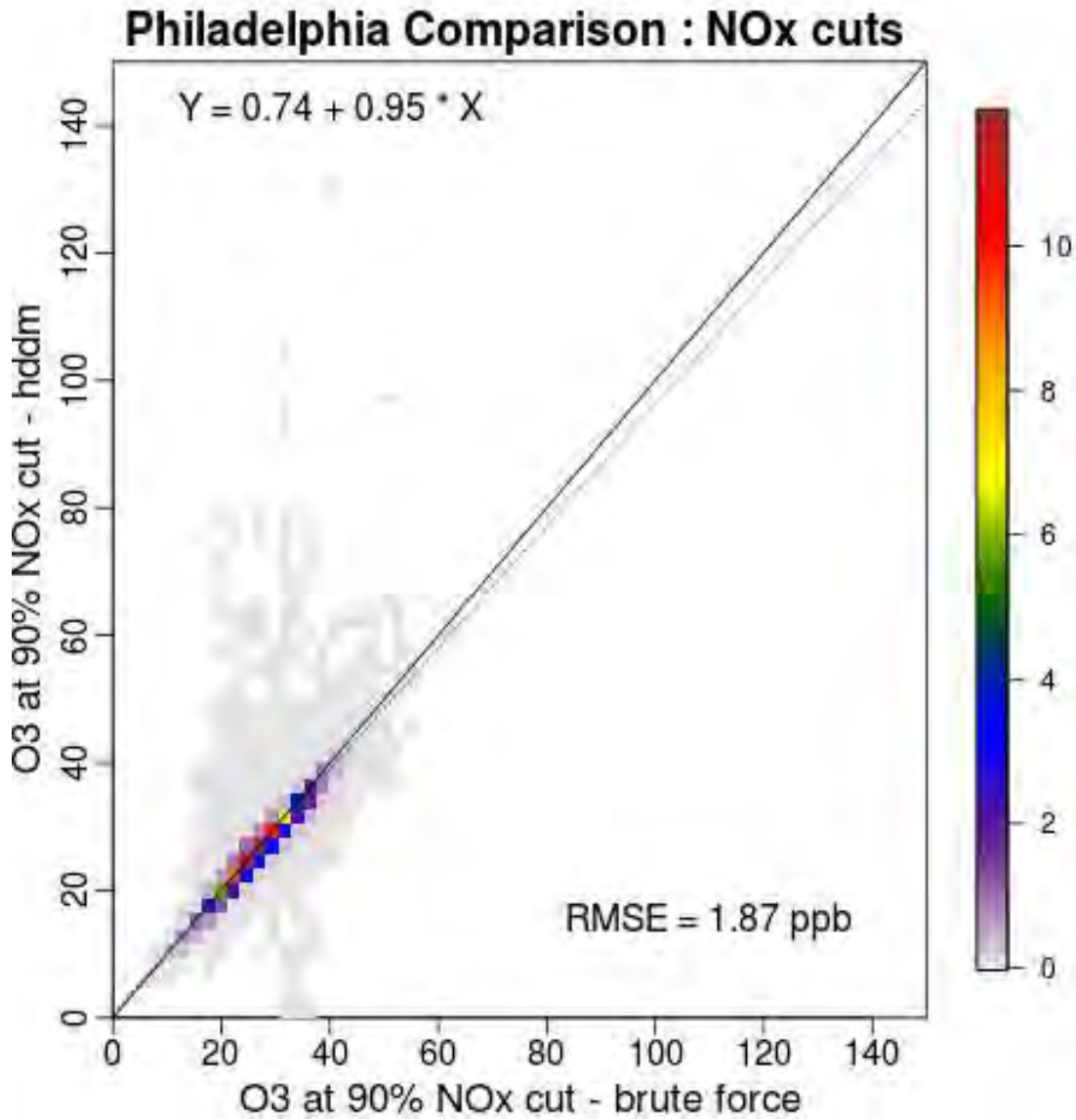
2 Figure 3C-62. Comparison of brute force and 3-step HDDM O 3 estimates for 90% NO x 3 cut conditions in Philadelphia.
