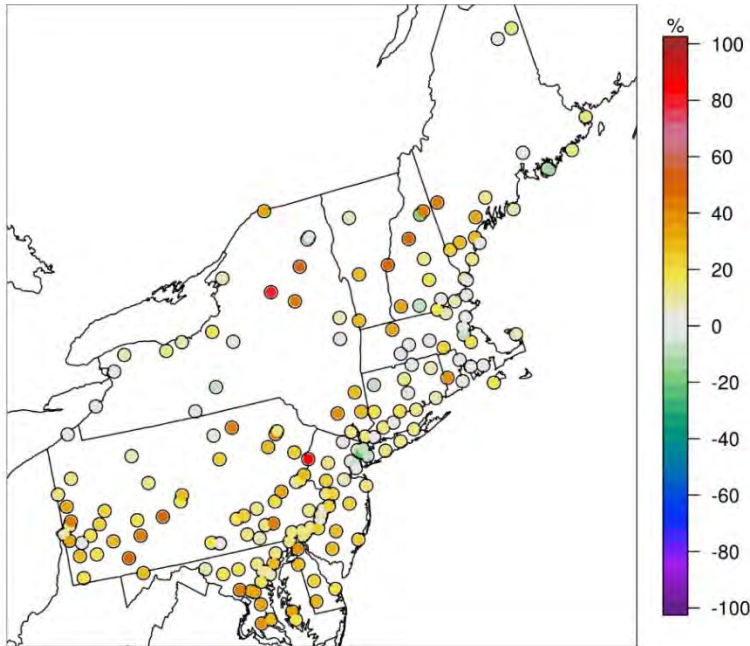
4 5 Figure 3C-14. Normalized mean bias for MDA8 O 3 in the Northeastern U.S., summer 6 2016.
