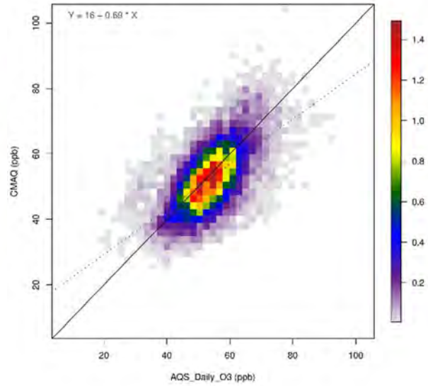
CMAQ_2016fe_cb6r3_16j_12US2 O3_8hrmax for Summer_Southwest
