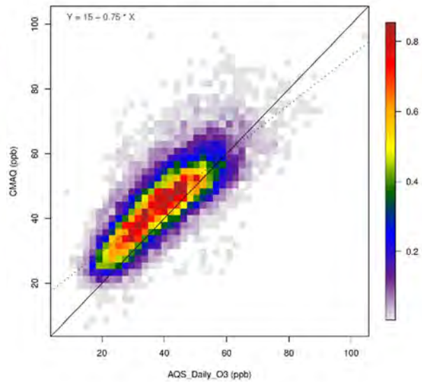
CMAQ_2016fe_cb6r3_16j_12US2 O3_8hrmax for Summer_Southeast
