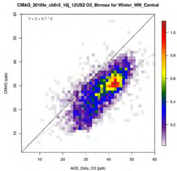
5 Figure 2B-10. Density scatter plots of observed versus predicted MDA8 O 3 from the 12km 6 resolution CONUS simulation for the WestNorthCentral region by season. 7 Each plot has a separate scale that is shared for the x and y axes. The dashed line 8 represents the best fit linear regression line.
