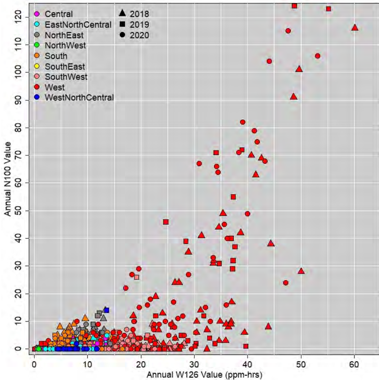
1 2 Figure 4F-10. Scatter plot of annual N100 values (Y-axis) versus annual W126 values (x- 3 axis), based on 2018-2020 monitoring data. 4
