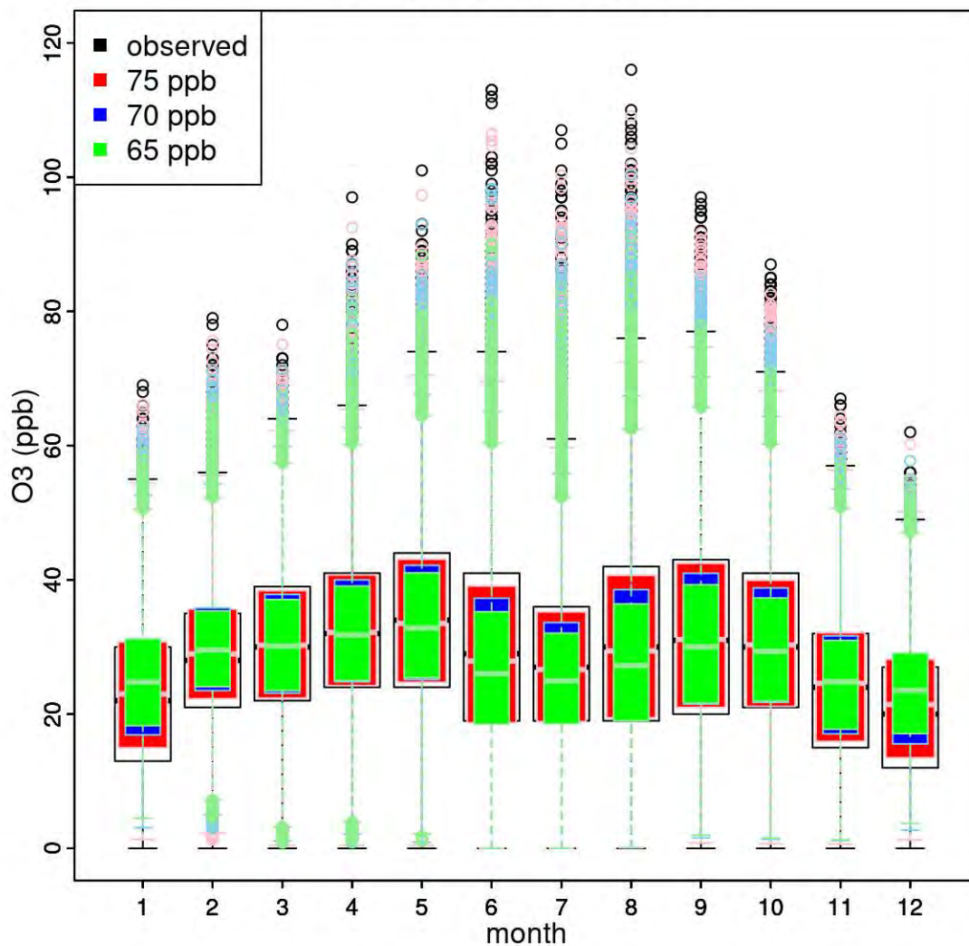
1 2 Figure 3C-77. Monthly distribution of hourly O 3 concentrations at monitoring sites in the 3 Dallas study area.
