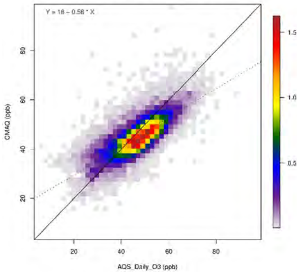
CMAQ_2016fe_cb6r3_16j_12US2 O3_8hrmax for Spring_Southeast
