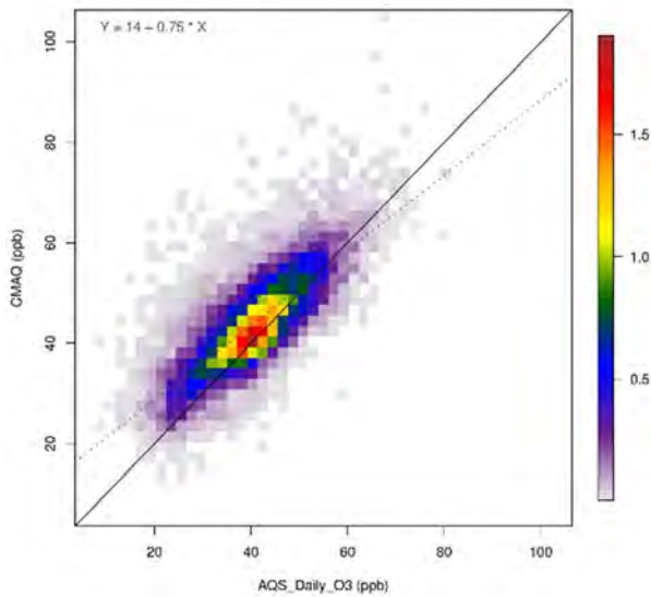
CMAQ_2016fe_cb6r3_16j_12US2 O3_8hrmax for Fall_Southeast
