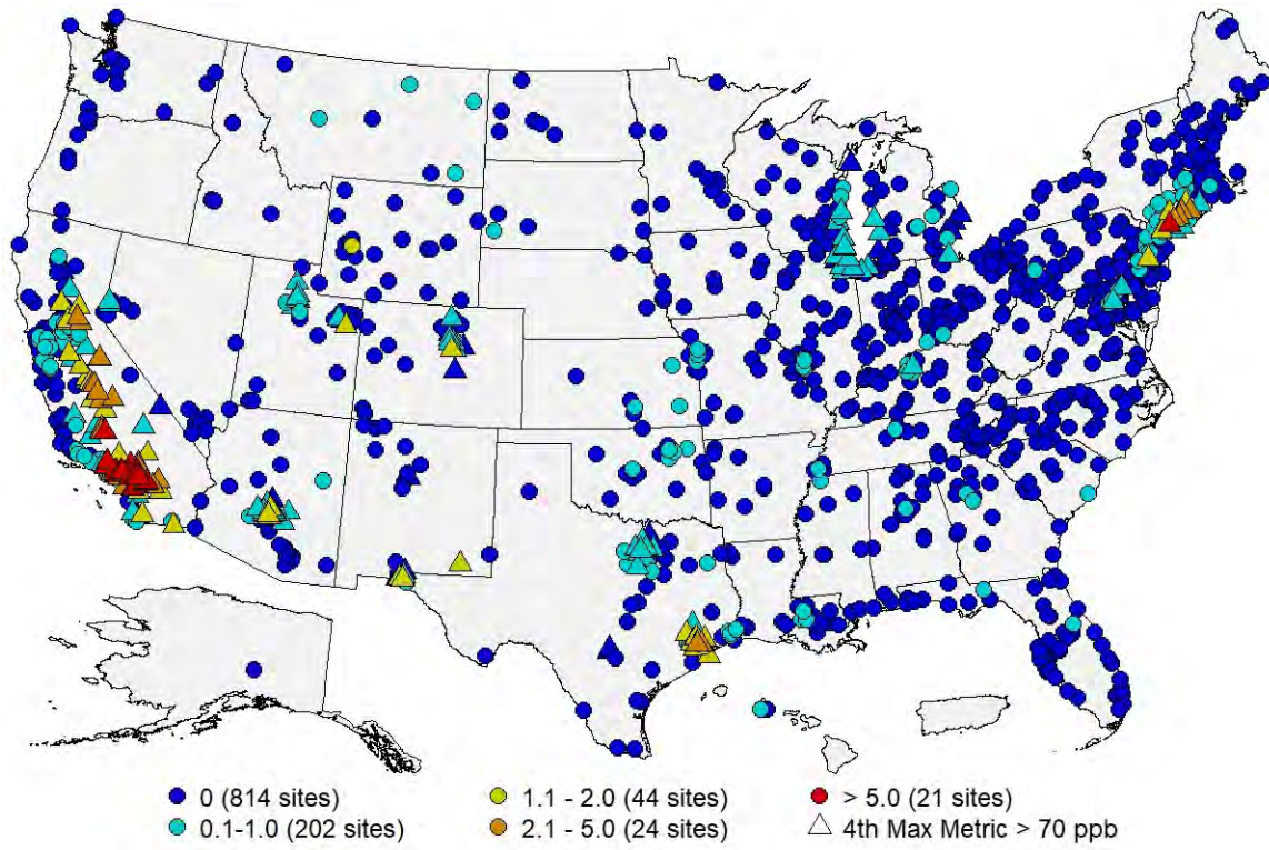
3 Figure 4F-3. Map of 2018-2020 Average D100 Values at sites with valid design values.
